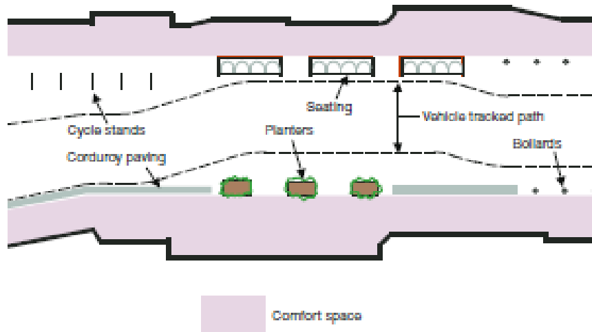
Figure 6.7 Comfort space
